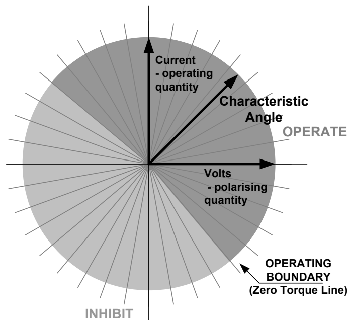
Figure 2.7-1 Directional Characteristics
