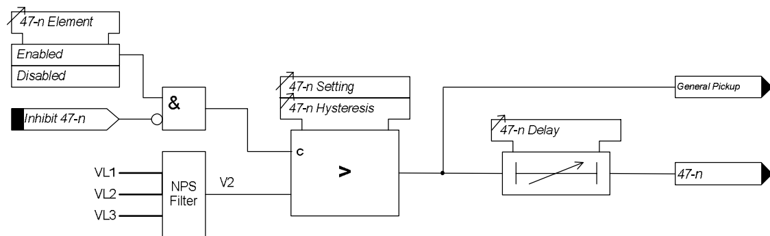
Figure 3-28 Logic Diagram: NPS Overvoltage Protection (47)
