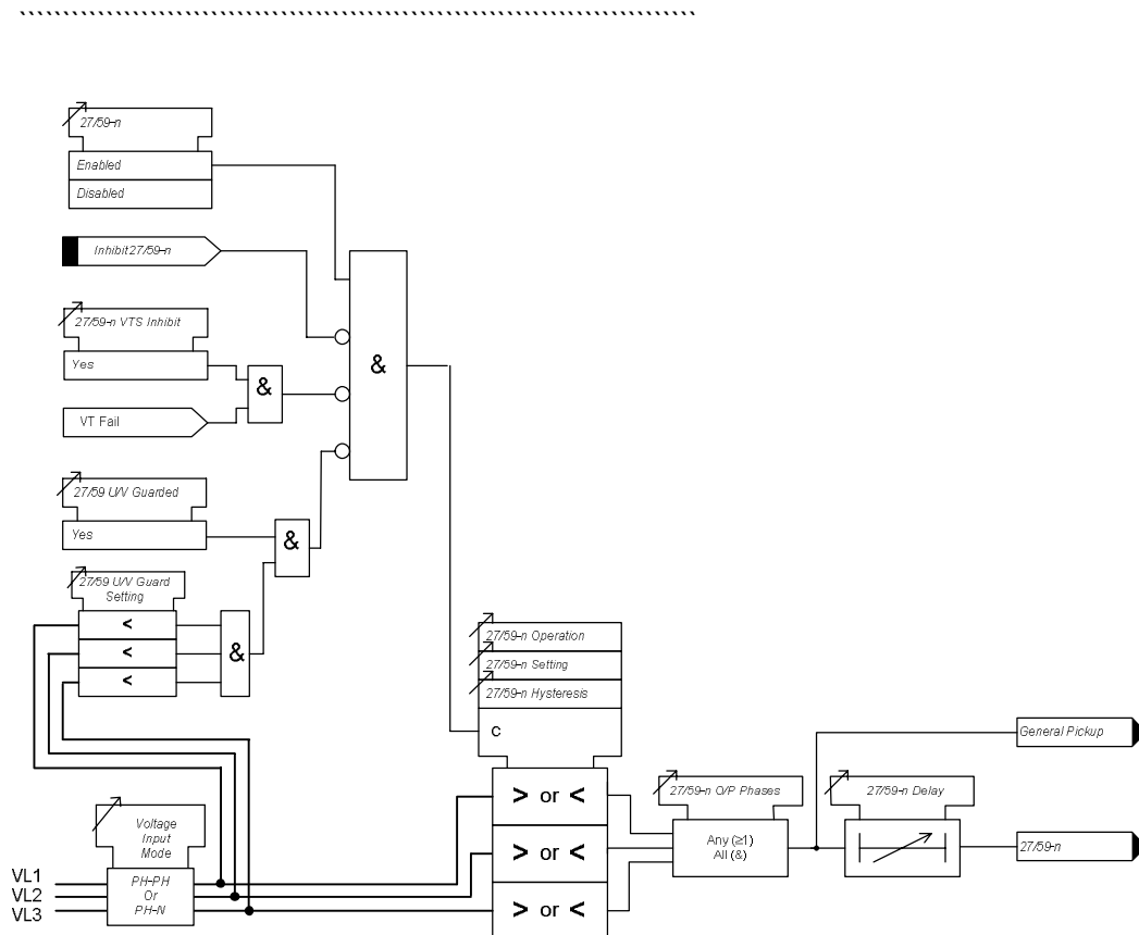
Figure 3-27 Logic Diagram: Under/Over Voltage Elements (27/59)
