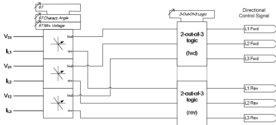
Figure 3-1 Logic Diagram: Directional Overcurrent Element (67)
