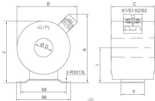
FIG.1 CG-PVB
