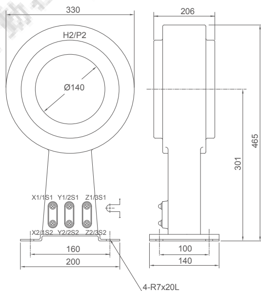
FIG.2 CGT-2MV
