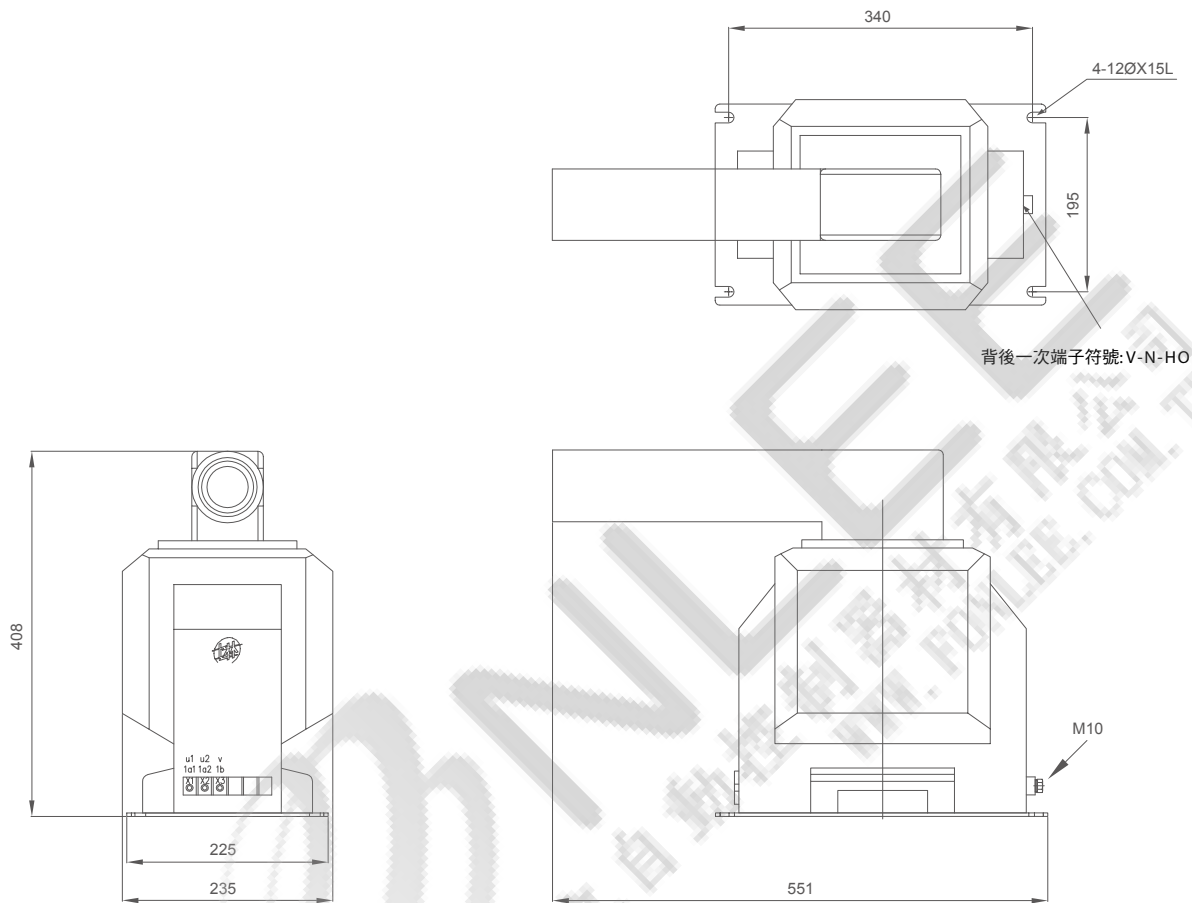
FIG.1 EMS-24D
