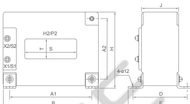
FIG.2 CG-QV
