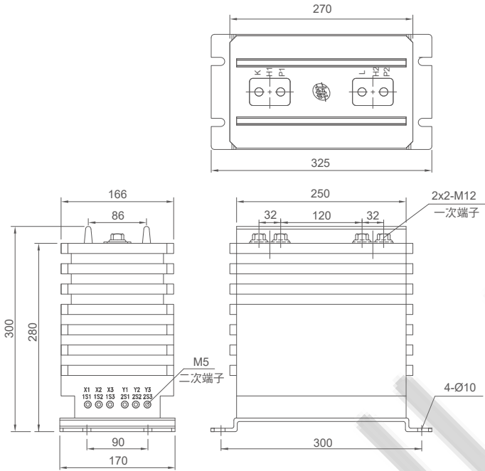
FIG.1 CMD-2KH
