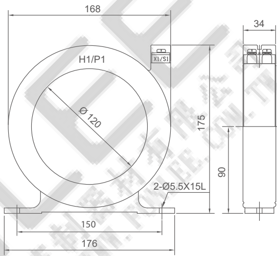
FIG.3 CG-PVB
