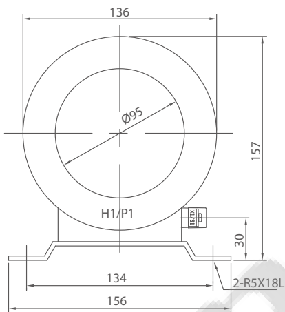
FIG.2 CG-JVA
