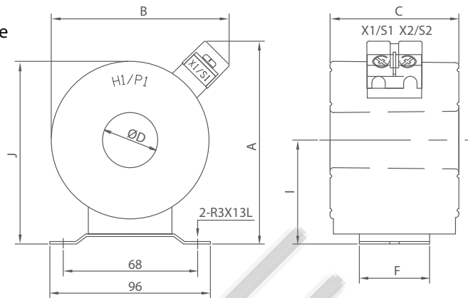
FIG.1 CG-JVA
