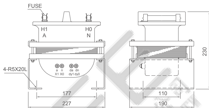
FIG.1 EHG-3ZF
