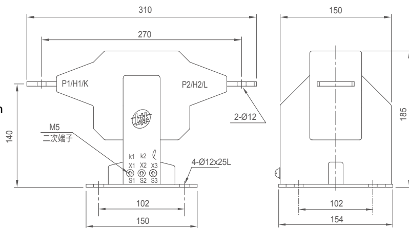
FIG.1 CM-1QV
