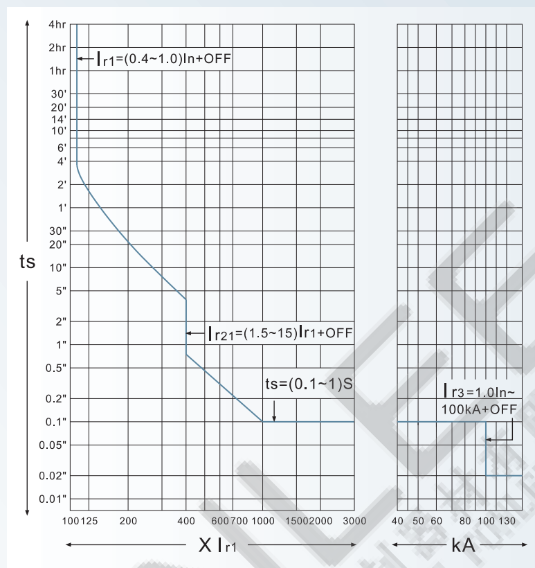
c.III 框動作曲線(BA4000-H、BA5000-H、BA6300-H)
