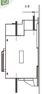
Busbar to Base Plate
