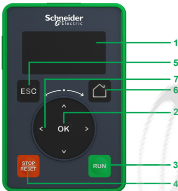
Plain text display terminal
