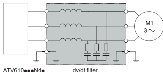
Altivar ATV610 drive with dv/dt filter
