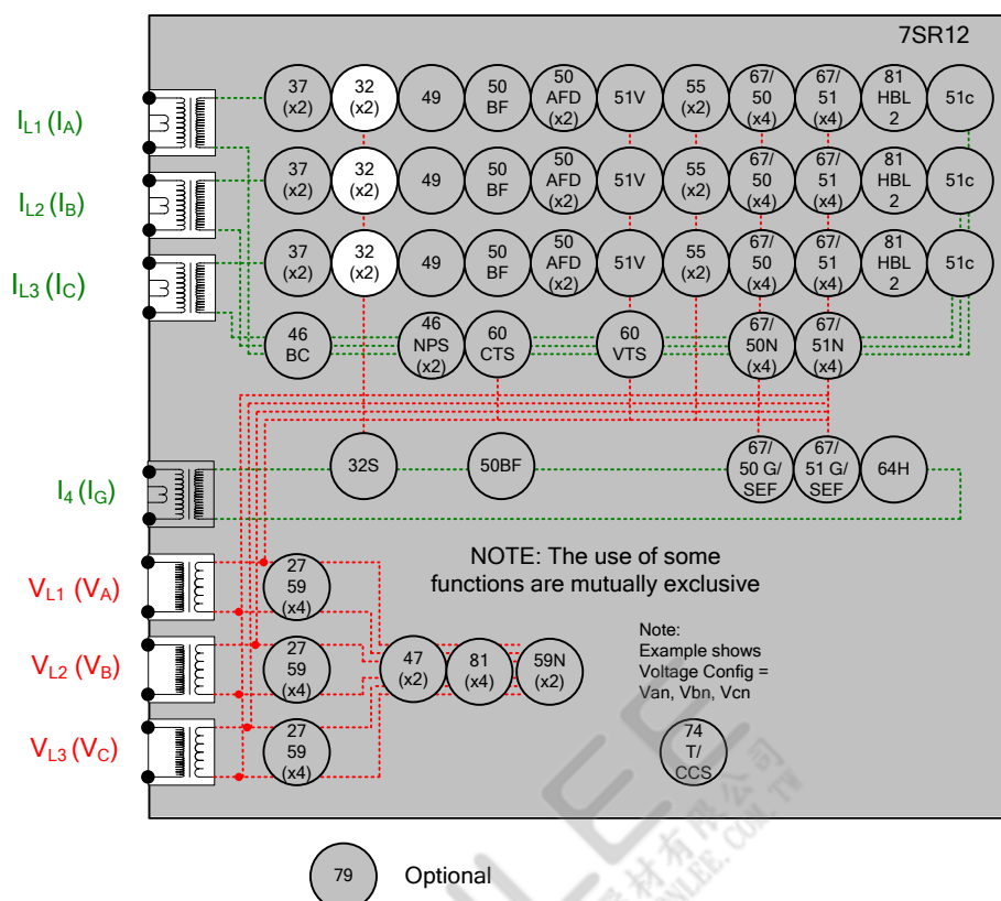
Figure 2-19 Power
