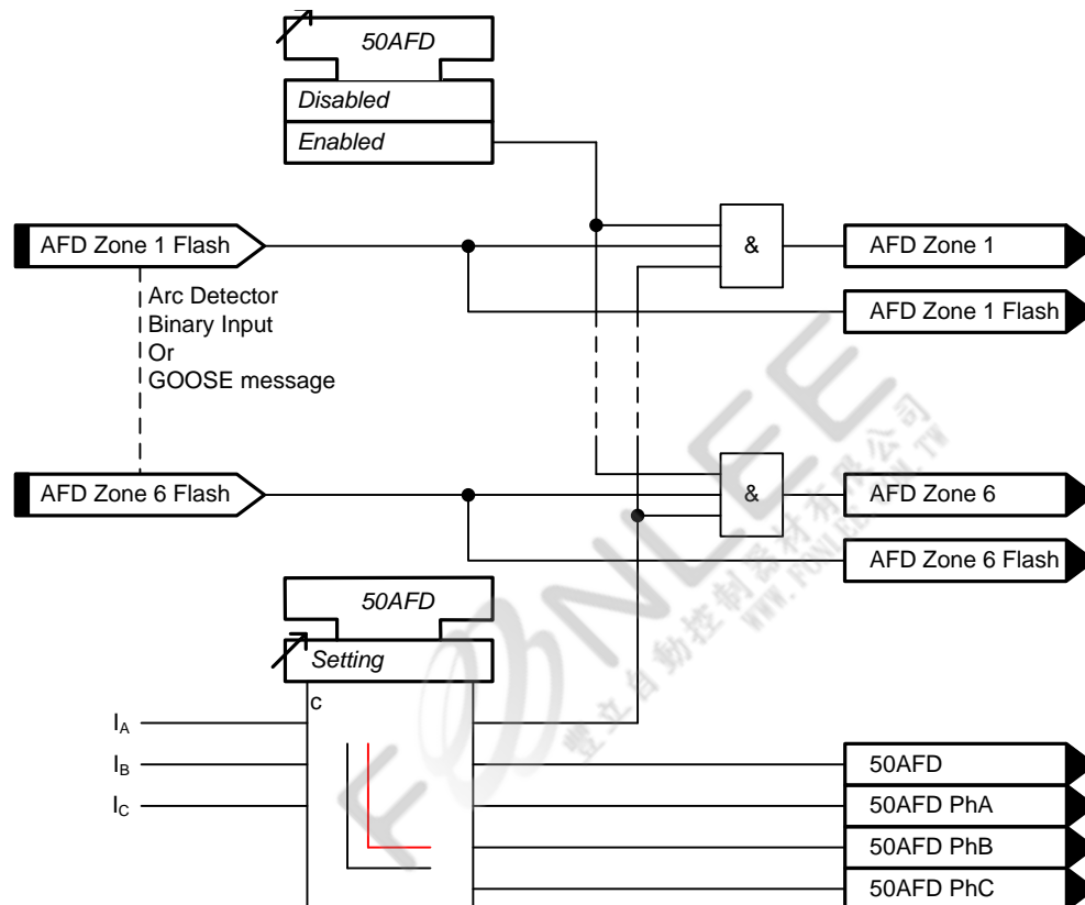
Figure 3-26 Logic Diagram: Arc Flash Detector (50 AFD)
