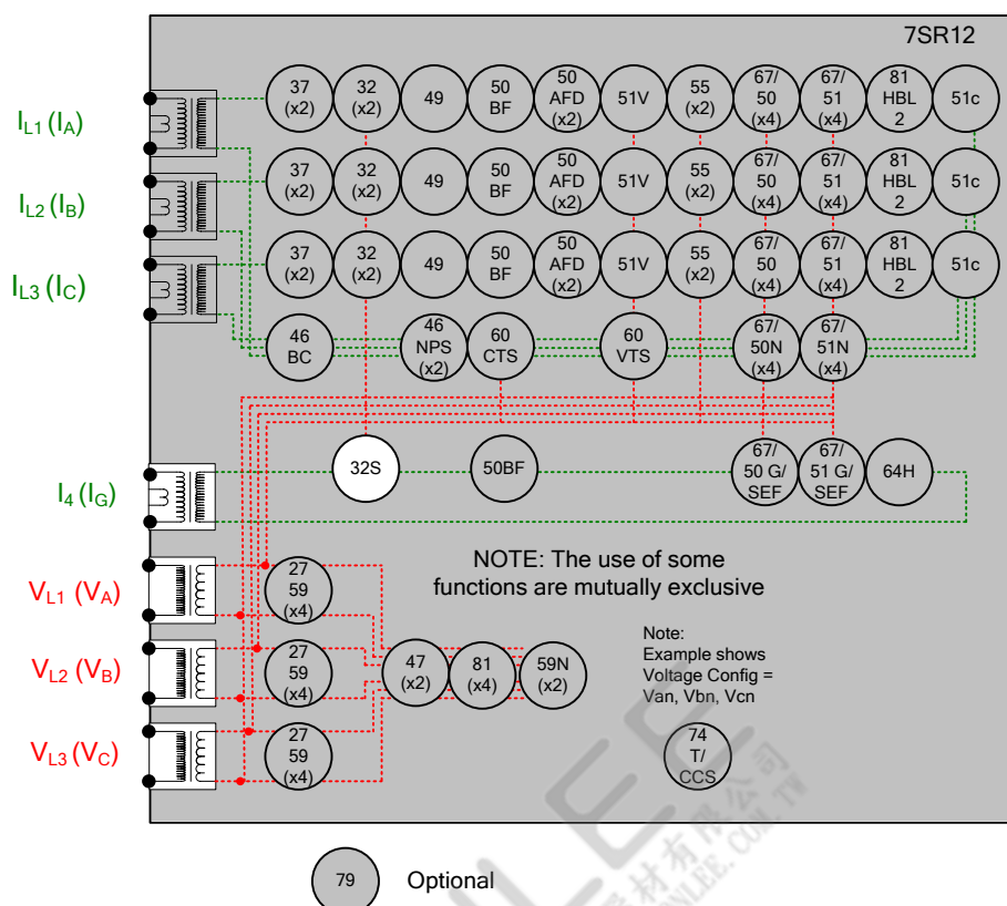
Figure 2-20 Sensitive Power
