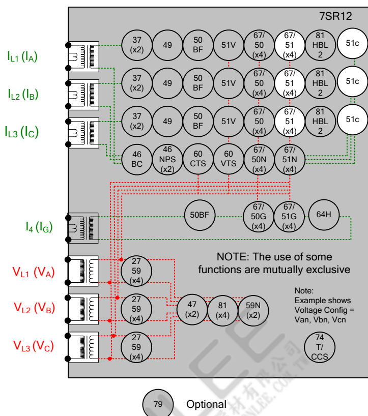
Figure 2-4 Cold Load
