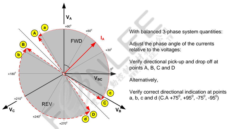
Figure 2-1 Directional Phase Fault Boundary System Angles
