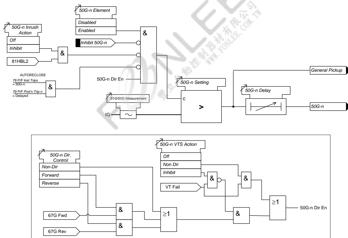
Figure 3-9 Logic Diagram: Measured Instantaneous Earth-fault Element
