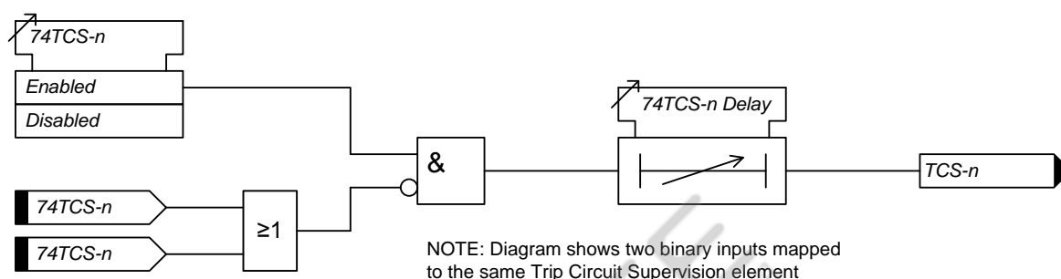
Figure 5-6 Logic Diagram: Trip Circuit Supervision Feature (74TCS)
