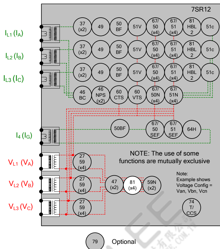
Figure 2-18 Under/Over Frequency
