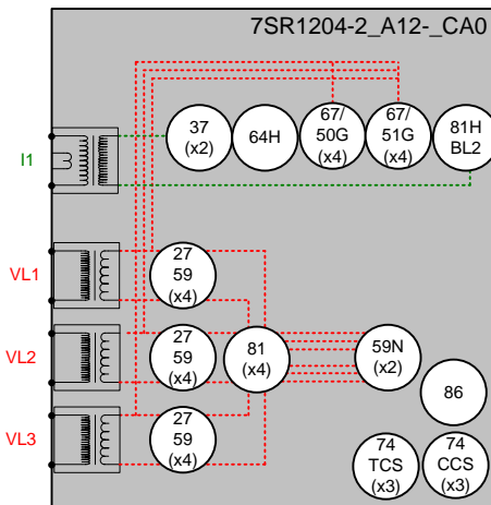
Figure 1-6 Functional Diagram of 7SR1204-2_A12-CA0 Relay
