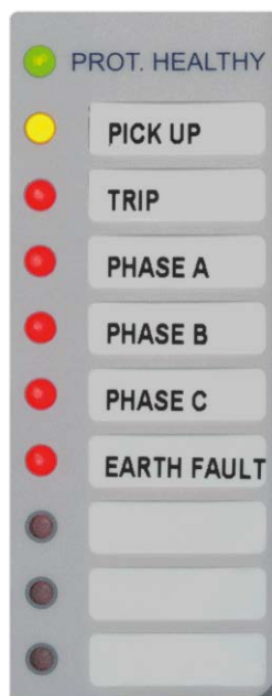
Figure 2-9 LED Indication Label
