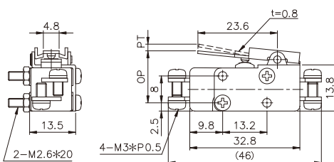
TW-1012B
