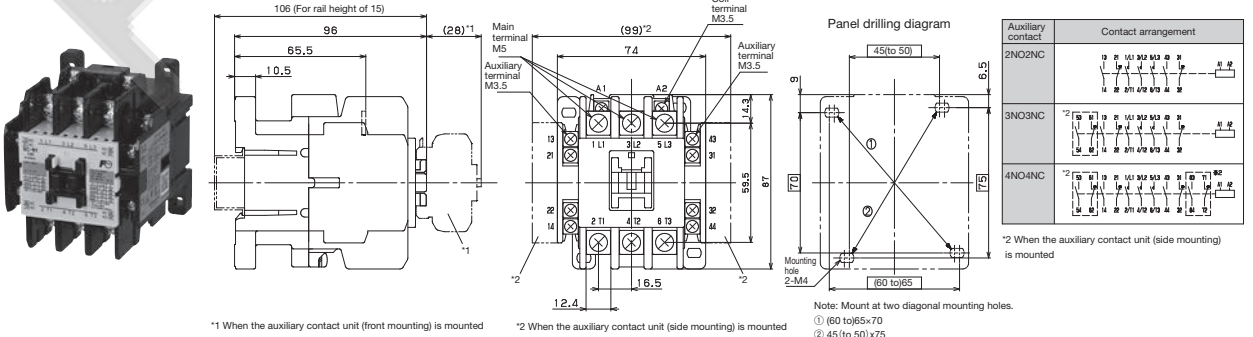
Outline drawing, wiring diagram
