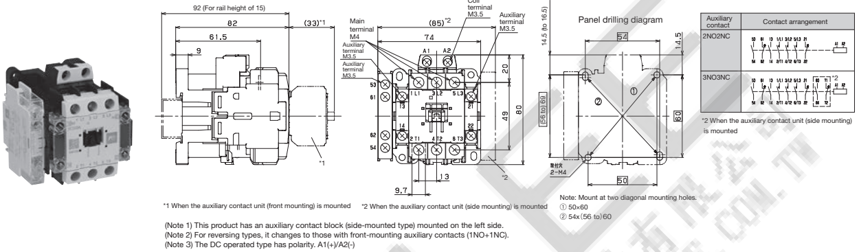
Outline drawing, wiring diagram
