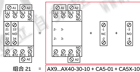
组合 21 = AX9...AX40-30-10 + CA5-01 + CA5X-10
