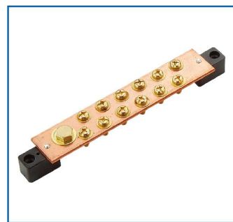
WJ-9112 動力端子板 12P Grounding Terminal Plate Power
