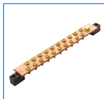
WJ-9120 動力端子板 20P Grounding Terminal Plate Power
