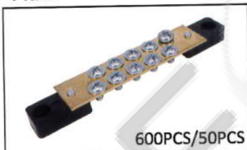
WJ-9009 接地端子板 9P Grounding Terminal Plate
