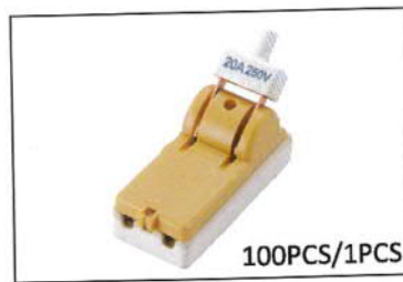
KS-2220 單投開關 2P20A 250V Knife Switch Single Throw
