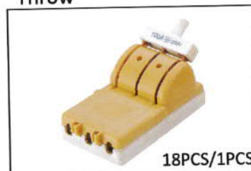
KS-3100 單投開關 3P100A 250V Knife Switch Single Throw
