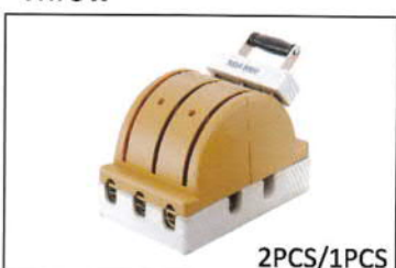
DKS-3300-1 雙投開關 3P300A 600V Knife Switch Double Throw
