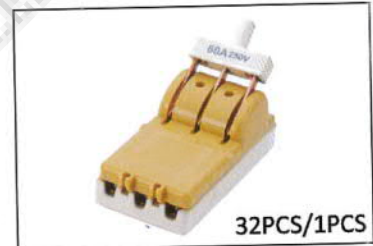
KS-3360 單投開關 3P60A 250V Knife Switch Single Throw
