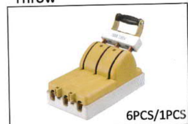
KS-3150 單投開關 3P150A 380V Knife Switch Single Throw
