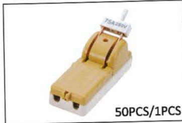
KS-2275 單投開關 2P75A 250V Knife Switch Single Throw
