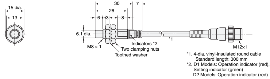
Diagram 30 E2E-X4MD□-M1TGJ-US
